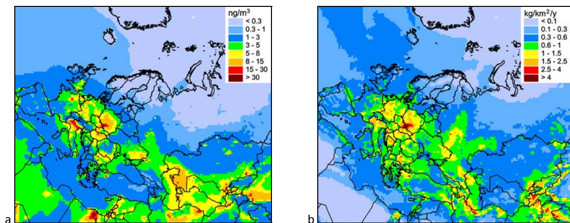
Fig. 1.10. Mean annual air concentrations (a) and total deposition (b) of lead in 2015
