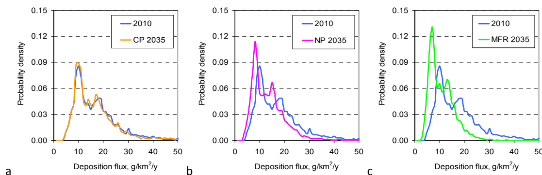
Fig. 4.17. Probability distribution of mercury deposition flux to forests of the Northern Hemisphere in 2035 in comparison with 2010 according to different emission scenarios: (a) – CP 2035; (b) – NP 2035; (c) – MFR 2035
