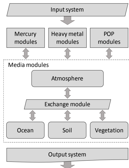
Fig. 2.1. General scheme of GLEMOS modules
