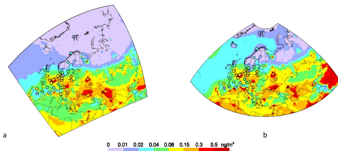
Fig. 2.7. Annual mean air concentration of Cd in 2014 simulated over the old (a) and new (b) EMEP domains. Coloured circles show Cd observations from the EMEP monitoring network
