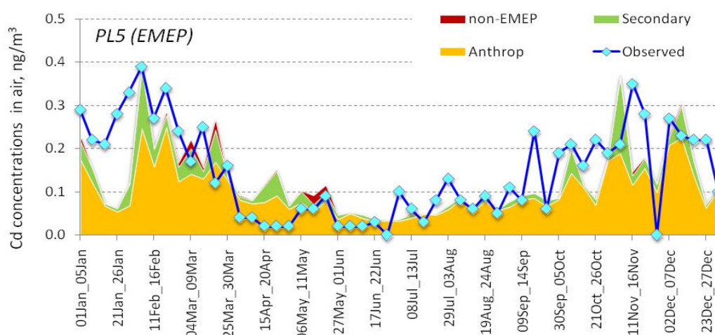
Fig. 3.16. Time series of modelled and observed concentrations of cadmium at the EMEP station PL5 (Diabla Gora) in 2014
