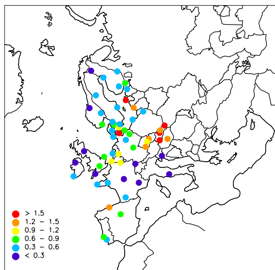
Fig. 1.4. Pb in precipitation, µg/L
