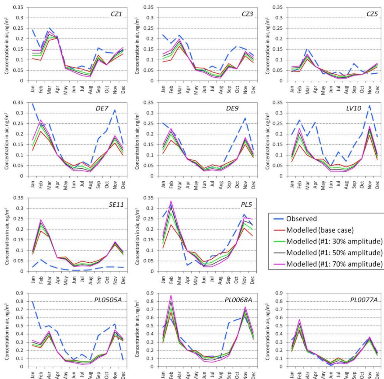
Fig. 3.10. Monthly mean cadmium air concentrations observed at Polish background regional and EMEP stations and modelled using scenarios of emission seasonal variability
