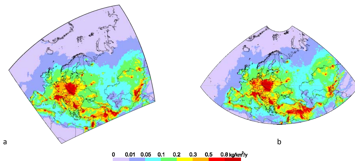
Fig. 2.3. Annual Pb deposition flux in 2014 simulated over the old (a) and new (b) EMEP domains
