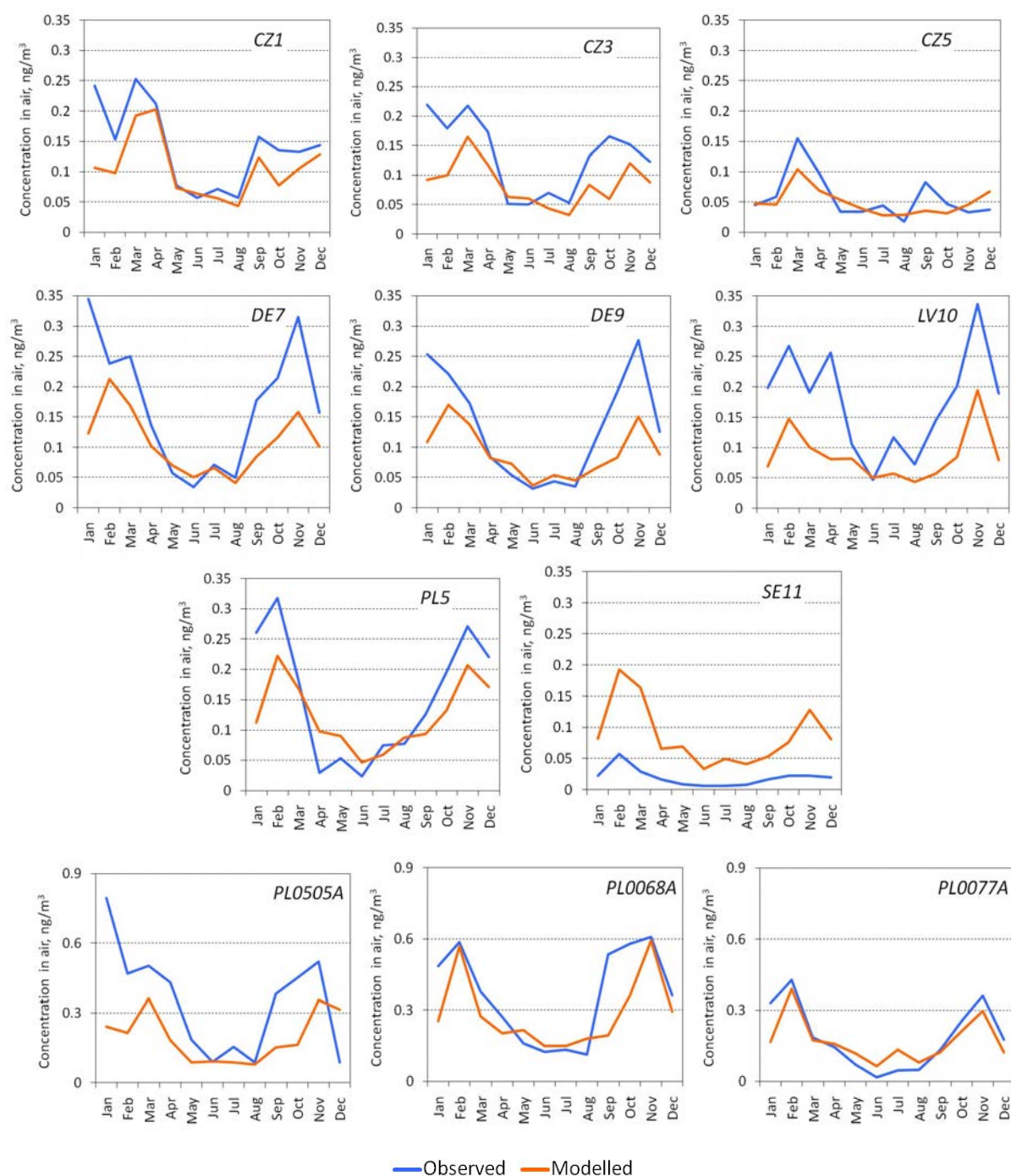
Fig. 3.8. Monthly mean modelled and observed concentrations of cadmium in air in 2014 at EMEP and national (background regional and suburban) Polish stations
