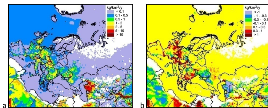
Fig. 1.19. Wins re-suspension flux of lead in 2015 (a) and difference between re-suspension fluxes in 2015 and 2014. Positive values of the difference mean increase, and negative – decrease of the flux in 2015 compared to 2014
