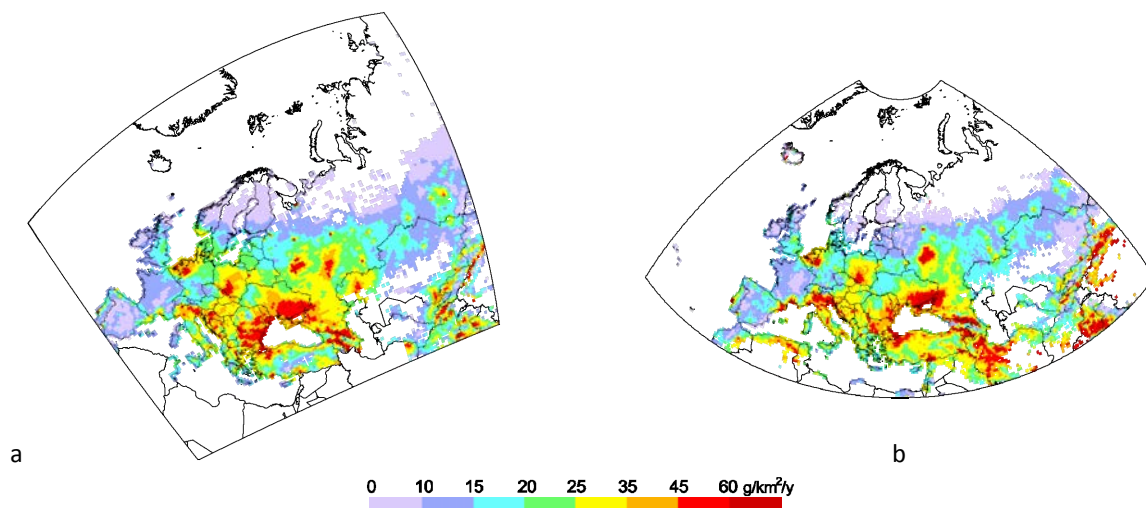
Fig. 2.10. Annual Cd deposition flux to croplands in 2014 simulated over the old (a) and new (b) EMEP domains
