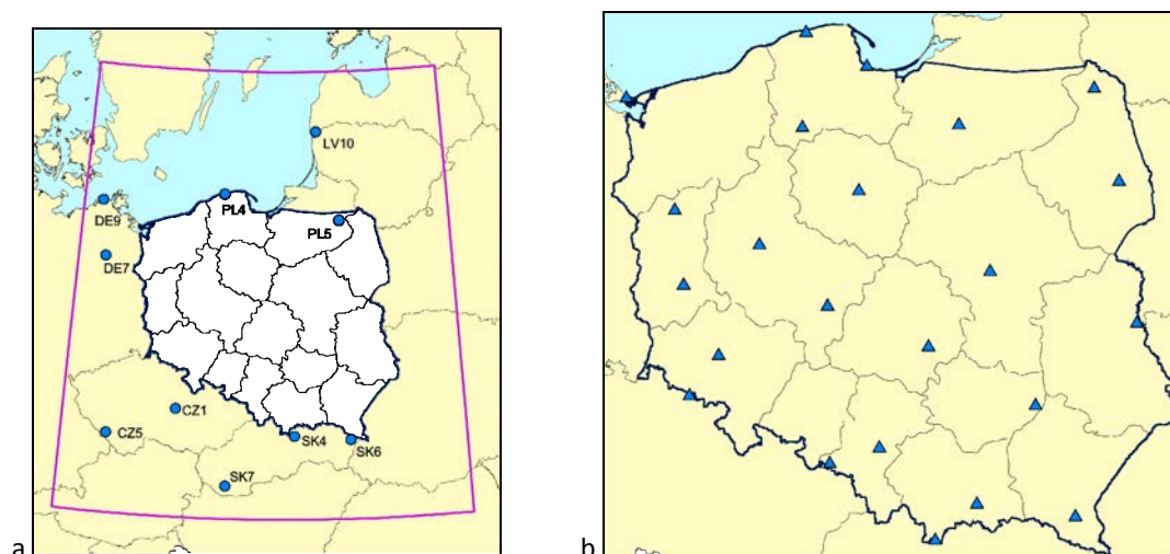
Fig. 3.5. Location of stations measuring wet deposition fluxes of cadmium at the EMEP network (a) and national Polish network (b)
