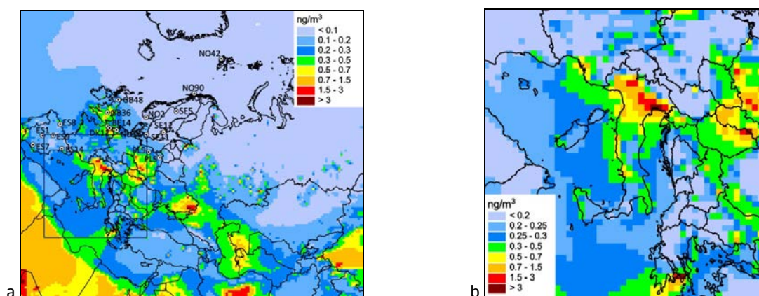
Fig. 4.2. Spatial distribution of annual mean concentrations of arsenic over EMEP domain (a) and over the region for MINNI modelling (b) in 2015
