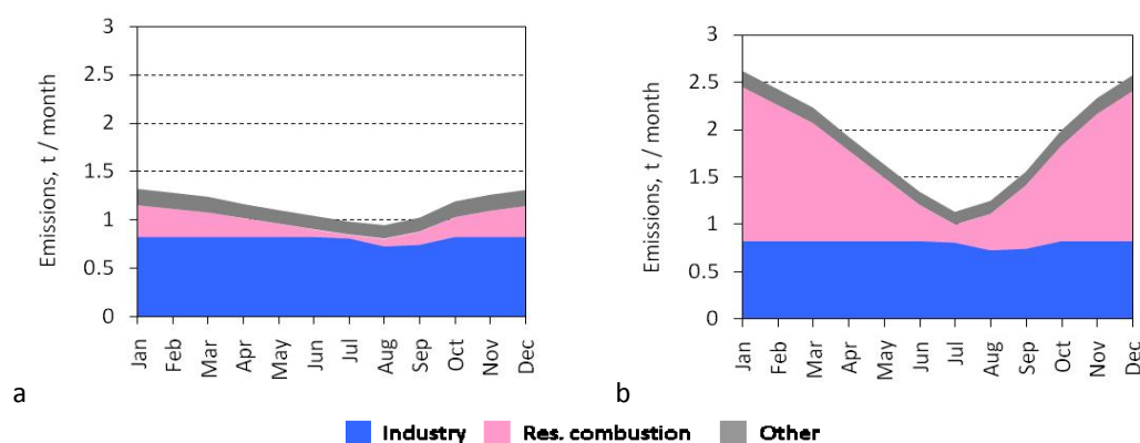
Fig. 3.14. Seasonal changes of cadmium emission data in Poland with original (a) and 5-fold increased (b) contribution of emission from residential combustion sector
