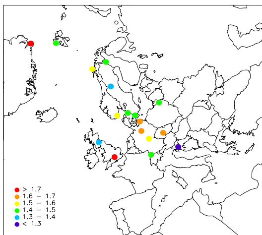
Fig. 1.7. Hg (g) in air, ng/m 3
