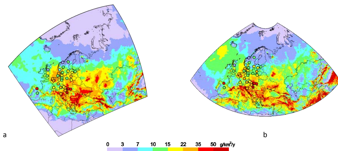
Fig. 2.8. Annual Cd wet deposition flux in 2014 simulated over the old (a) and new (b) EMEP domains. Coloured circles show Cd observations from the EMEP monitoring network
