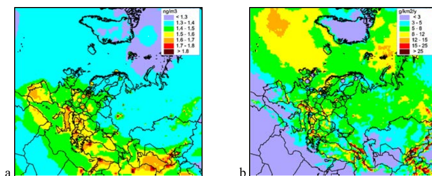
Fig. A.3. Spatial distribution of modelled and observed mercury concentrations in air (a) and wet deposition fluxes (b) in 2015
