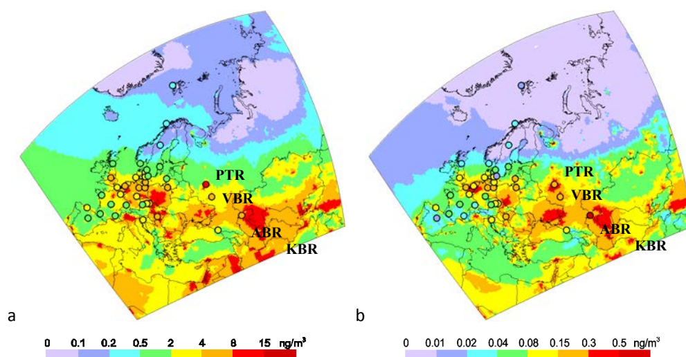
Fig. 4.9. Modelled and observed annual mean concentrations of lead (a) and cadmium (b) in the EMEP region in 2014
