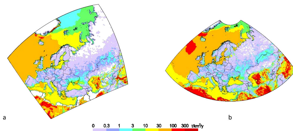
Fig. 2.5. Mineral dust (PM10) suspension from natural surfaces in 2014 simulated over the old (a) and new (b) EMEP domains
