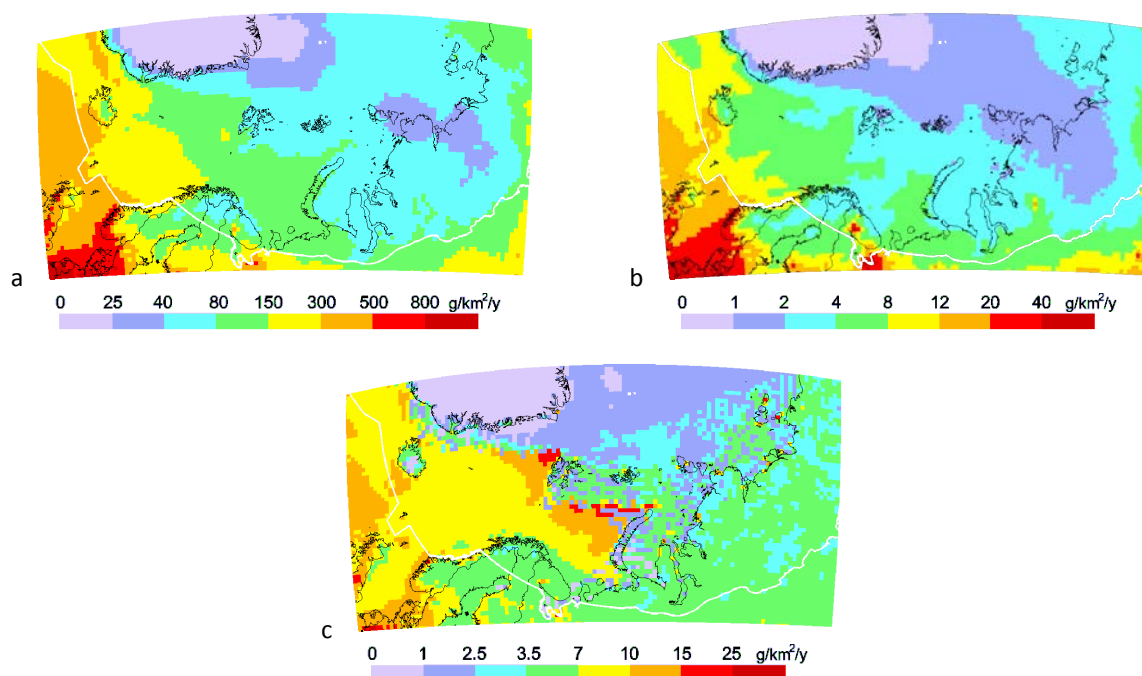
Fig. 1.24. Spatial distribution of annual total deposition of lead (a), cadmium (b) and net deposition flux of mercury (c) over the Arctic sector of the EMEP region in 2014. White line depicts the boundary of the AMAP domain
