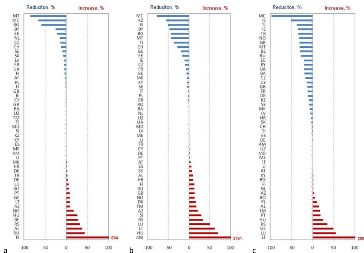
Fig. 1.1. Relative changes of annual total emissions of lead (a), cadmium (b) and mercury (c) between 2014 and 2015, %
