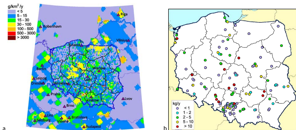
Fig. 3.2. Spatial distribution of cadmium emission in the modelling domain (a) and distribution of emissions from LPS in Poland (b)
