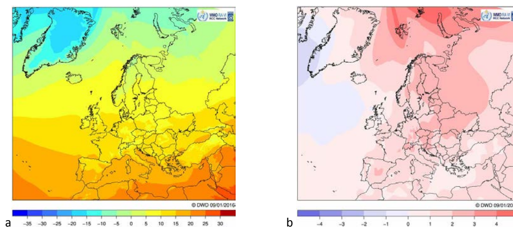
Fig. B.1. Annual mean air temperature (a) and its anomaly (b) for 2015, °C, relative to period of 1961-1990.
