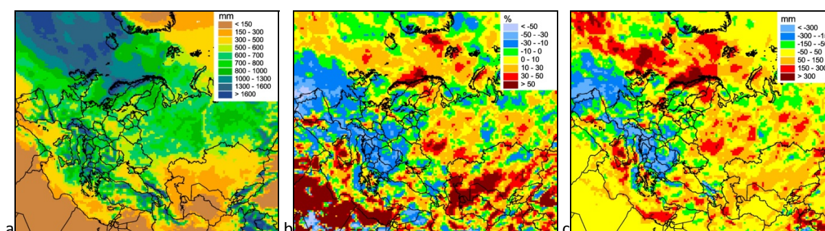
Fig. 1.18. Precipitation amounts in 2015 (a) and relative (b) and absolute (c) difference between precipitation in 2015 and 2014 (b). Positive values of the difference mean increase, and negative – decrease of precipitation in 2015 compared to 2014
