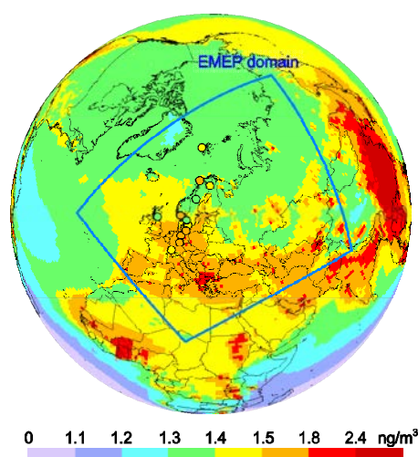
Fig. 1.9. Global distribution of Hg^0 concentration in 2015. Blue line depicts the boundary of the EMEP domain. Circles show EMEP measurements in the same color palette
