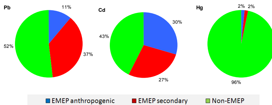
Fig. 1.25. Average contribution of different source types to annual deposition of lead (a), cadmium (b), and mercury (c) to the European and Asian terrestrial areas of the Arctic covered by the EMEP domain
