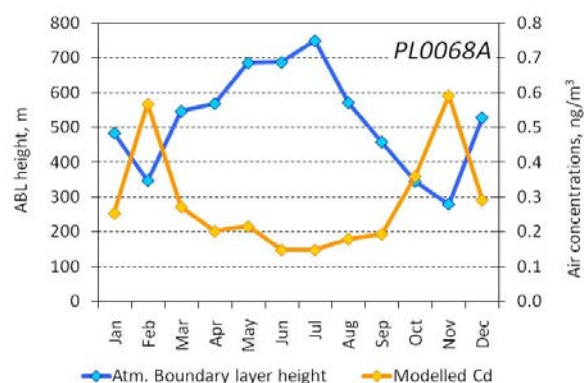
Fig. 3.9. Monthly mean values of atmospheric boundary layer height and cadmium concentrations in air at national Polish station PL0068A
