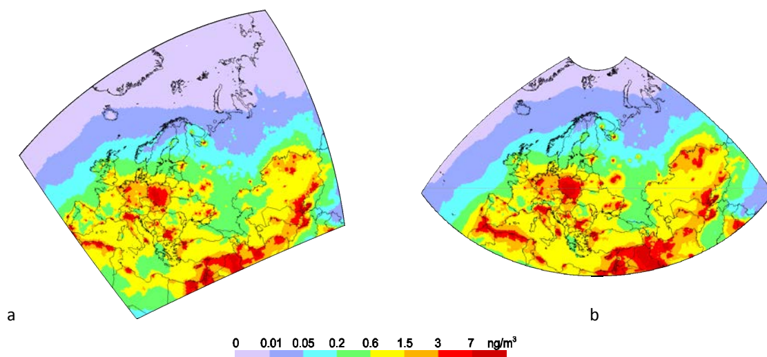
Fig. 2.2. Annual mean air concentration of Pb in 2014 from anthropogenic sources simulated over the old (a) and new (b) EMEP domains
