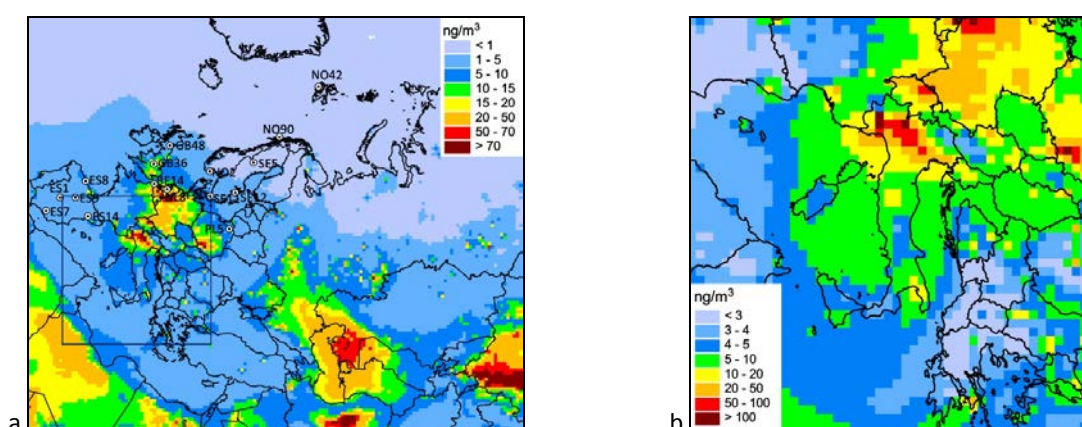
Fig. 4.3. Spatial distribution of annual mean concentrations of zinc over EMEP domain (a) and over the region for MINNI modelling (b) in 2015
