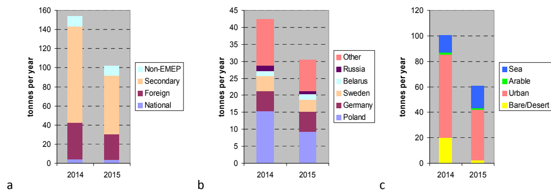
Fig. 1.20. Contribution of anthropogenic (national and foreign), secondary and non-EMEP sources to lead deposition (a), contribution of main anthropogenic sources (b) and contributions of different land-cover categories to deposition from secondary sources (c) in Sweden in 2014 and 2015
