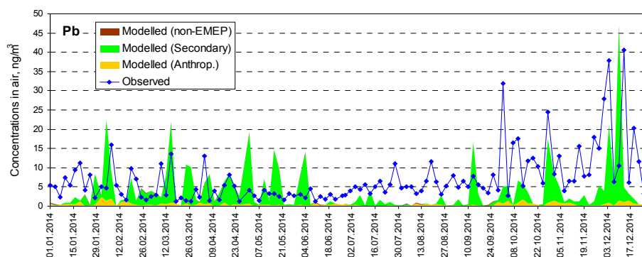
Fig. 4.11. Time series of modelled and observed concentrations of lead in air at station Voronezhsky Biosphere Reserve
