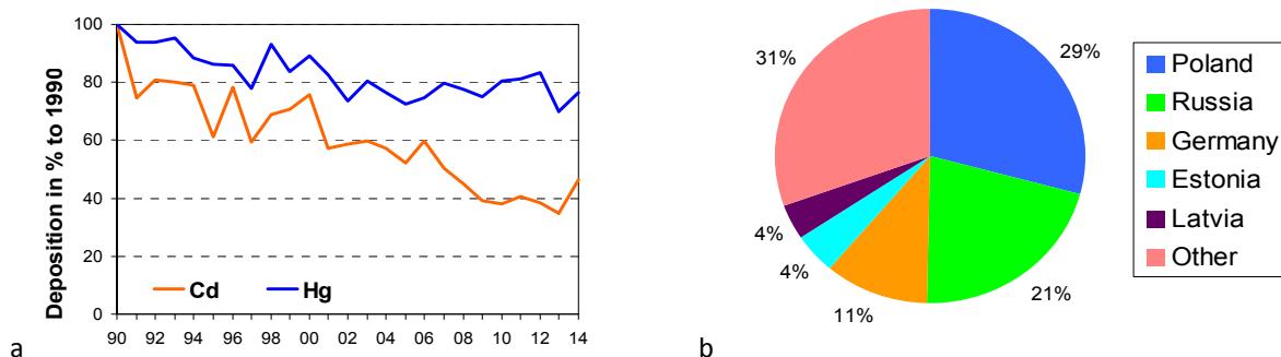
Fig. 4.18. Relative changes of annual atmospheric deposition of cadmium and mercury to the Baltic Sea in the period 1990-2014 (a) and contribution of emission sources from the EMEP countries to total anthropogenic deposition to the Baltic Sea in 2014 (b)
