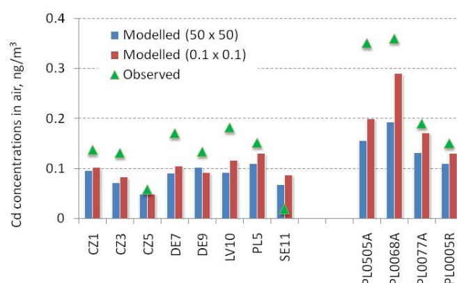
Fig. 3.7. Annual mean modelled (50x50 km 2 , 0.1°x0.1°) and observed concentrations of cadmium at the EMEP and national Polish background regional and suburban stations
