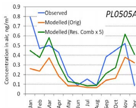
Fig. 3.15. Monthly-mean air concentrations of cadmium, modelled using different emissions form source category 'residential combustion' and observed at station PL0505A
