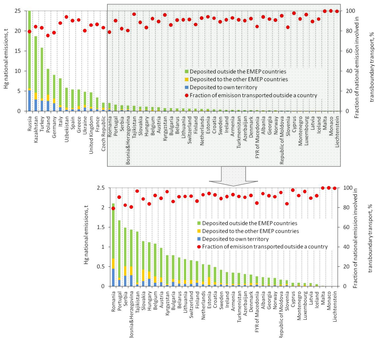
Fig. 1.14. Distribution of mercury emitted in the EMEP countries between deposition to own territory, deposition to the other EMEP countries and deposition outside the EMEP countries in 2015. Red dots indicate relative fraction of national emissions involved into the transboundary pollution
