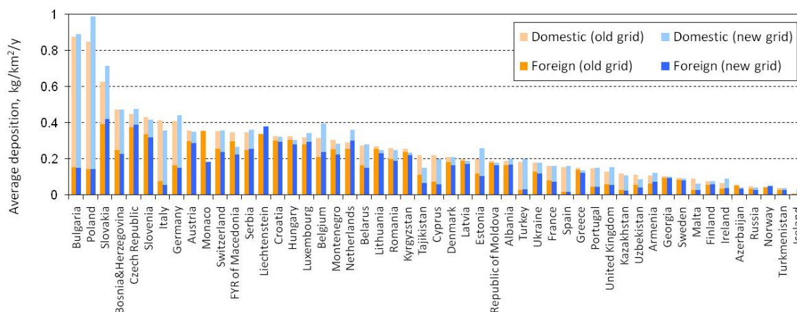
Fig. 2.4. Comparison of average Pb deposition from anthropogenic sources in the EMEP countries in 2014 simulated over the old and new domains
