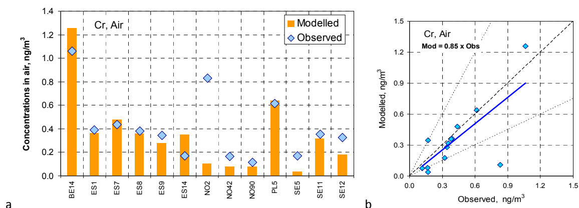
Fig. 4.6. Annual mean modelled and observed concentrations of chromium in air in 2015 at individual stations (a) and their scatter plot (b). Dashed line mean 1:1 ratio, and dotted lines mean 2-fold range
