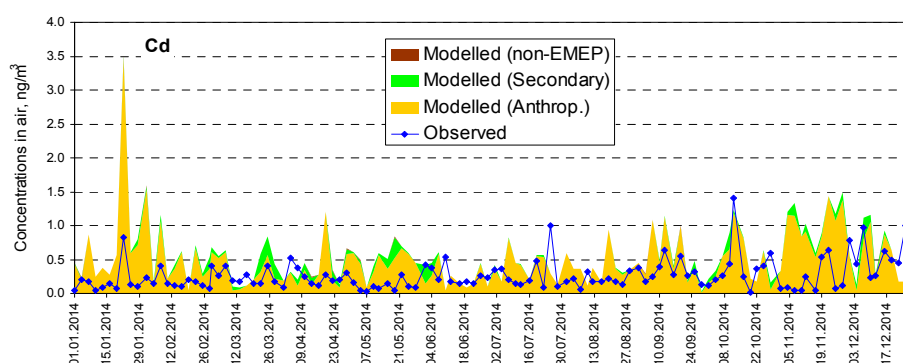
Fig. 4.12. Time series of modelled and observed concentrations of cadmium in air at station Prioksko-Terrasny Biosphere Reserve
