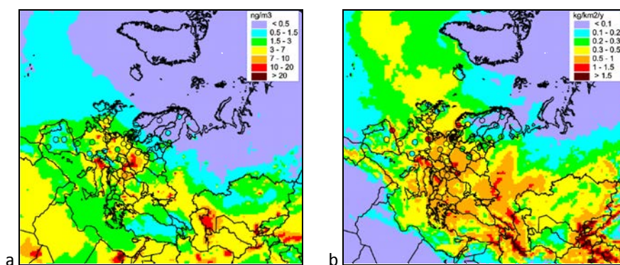
Fig. A.1. Spatial distribution of modelled and observed lead concentrations in air (a) and wet deposition fluxes (b) in 2015
