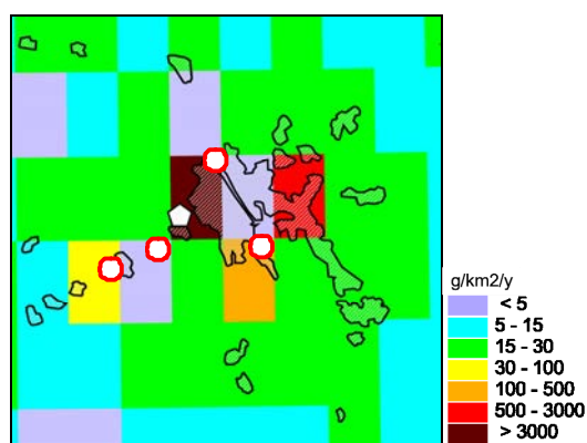
Fig. 3.20. Cadmium emission in Warsaw city and neighbouring areas. Pentagon indicates location of measurement station PL0214A, red circles – power stations
