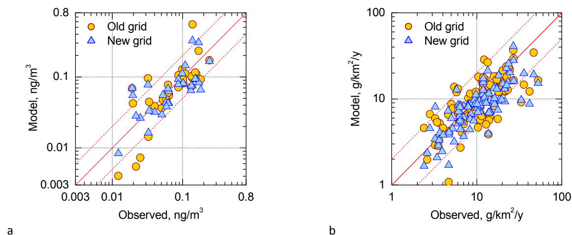
Fig. 2.9. Evaluation of annual mean air concentration (a) and wet deposition (b) of Cd in 2014 simulated over old and new EMEP domains against EMEP measurements
