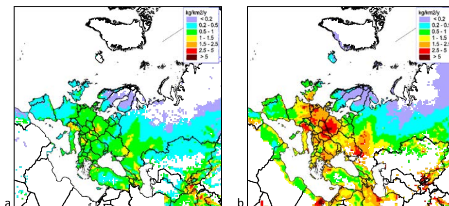
Fig. 4.15. Annual lead deposition flux to arable lands (a) and forest (b) in 2015
