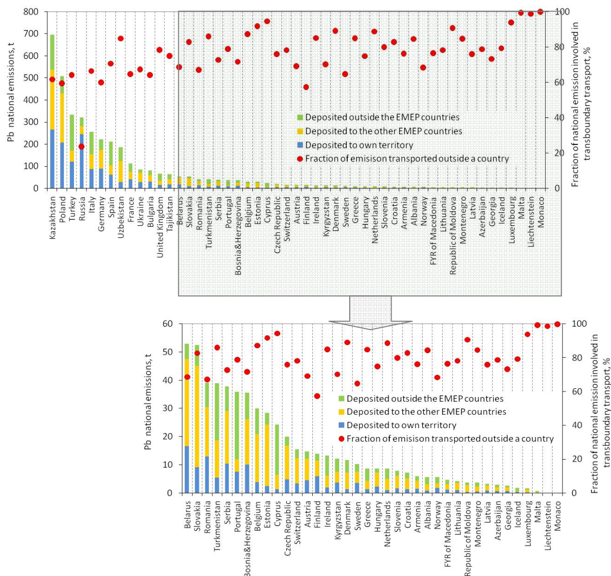
Fig. 1.13. Distribution of lead emitted in the EMEP countries between deposition to own territory, deposition to the other EMEP countries and deposition outside the EMEP countries in 2015. Red dots indicate relative fraction of national emissions involved into the transboundary pollution
