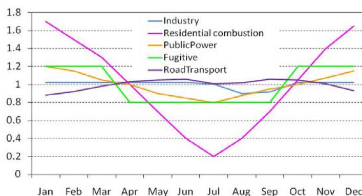
Fig. 3.11. Monthly factors applied to emission source categories, used in LOTUS/EUROS model
