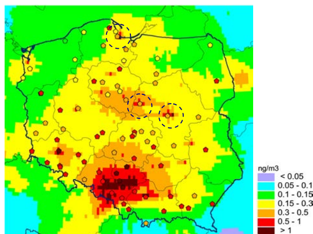
Fig. 3.19. Modelled (field) and observed (pentagons) concentrations of cadmium in air. Spatial resolution of calculated values is 0.1^\circ \times 0.1^\circ . Dashed circles indicate location of Warsaw, Gdansk and Plock
