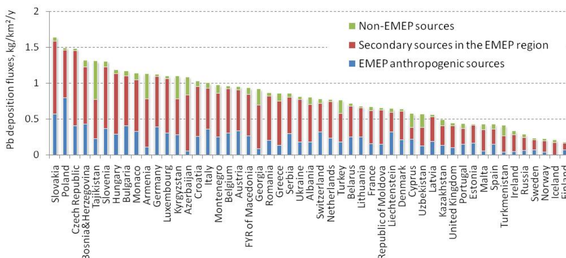
Fig. 1.11. Country-averaged deposition fluxes of lead from the European and Central Asian anthropogenic, secondary and non-EMEP emission sources in 2015
