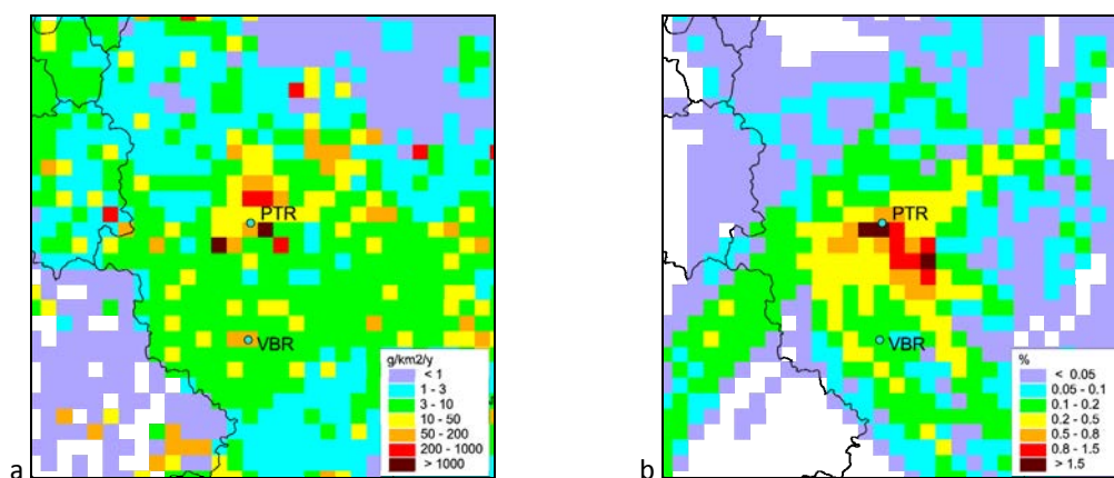
Fig. 4.13. Annual emission of cadmium (a) and HYSPLIT-based back trajectories (expressed as frequencies of trajectory presence in gridcells) for station Prioksko-Terrasny Biosphere Reserve for 01 st – 28 th of November
