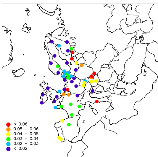
Fig. 1.6. Cd in precipitation, µg/L
