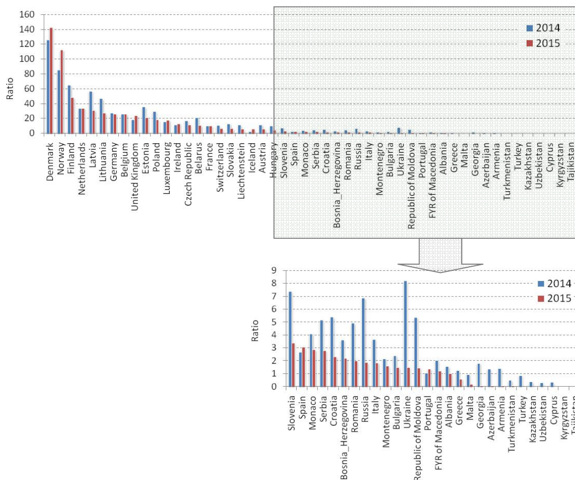
Fig. 1.21. Potential influence of foreign countries on lead deposition in Sweden in 2014 and 2015, expressed as a ratio of deposition from country's emission sources to country's emissions
