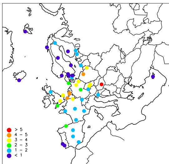
Fig. 1.3. Pb in aerosol, ng/m 3
