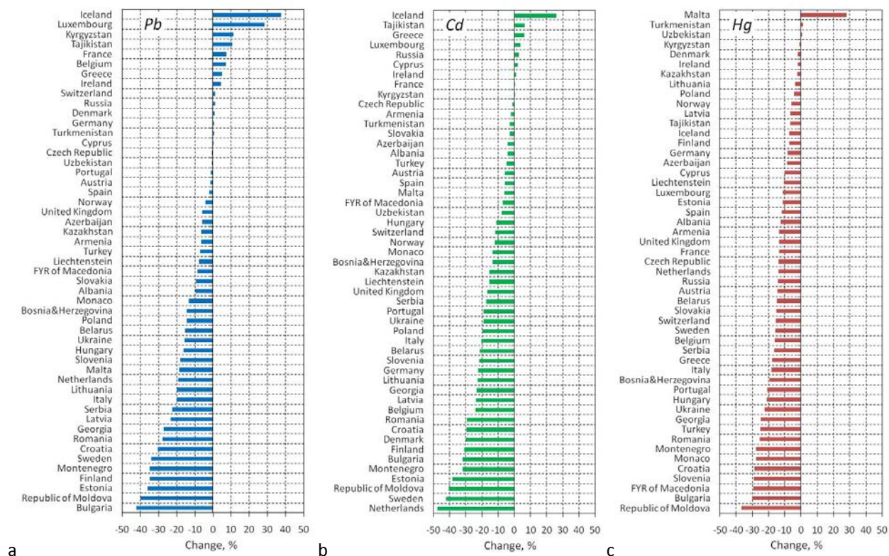
Fig. 1.15. Relative changes of lead (a), cadmium (b) and mercury (c) total deposition modelled for 2014 and for 2015
