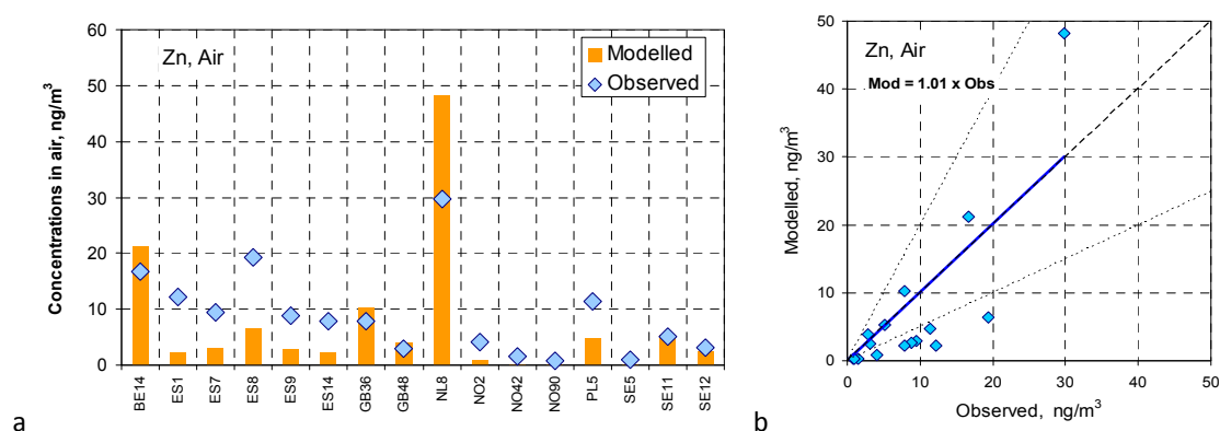
Fig. 4.7. Annual mean modelled and observed concentrations of zinc in air in 2015 at individual stations (a) and their scatter plot (b). Dashed line mean 1:1 ratio, and dotted lines mean 2-fold range
