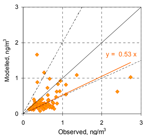
Fig. 3.18. Scatter plot of modelled ( 0.1^\circ \times 0.1^\circ ) and observed cadmium concentrations in air at urban stations for 2014. Dashed lines indicate factor of two range
