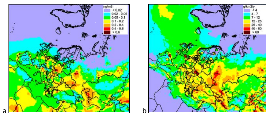
Fig. A.2. Spatial distribution of modelled and observed cadmium concentrations in air (a) and wet deposition fluxes (b) in 2015
