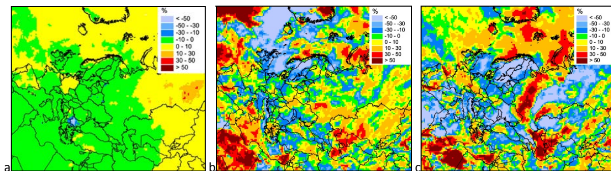
Fig. 1.17. Effects of lead deposition changes (% relative to 2015) between 2014 and 2015 caused by changes of reported anthropogenic emissions (a), meteorological conditions (b) and combined effect of meteorological data and wind re-suspension (c). Positive values mean increase of deposition from 2014 to 2015, and vice versa
