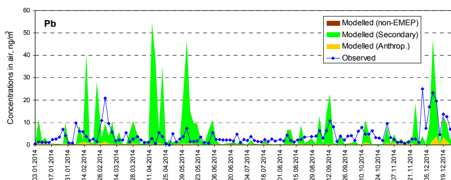
Fig. 4.14. Time series of modelled and observed concentrations of lead in air at station Astrakhansky Biosphere Reserve
