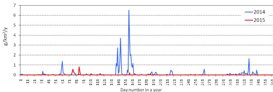
Fig. 1.22. Country-mean daily total deposition flux of lead caused by secondary sources from bare/desert lands in 2014 and 2015 in Sweden
