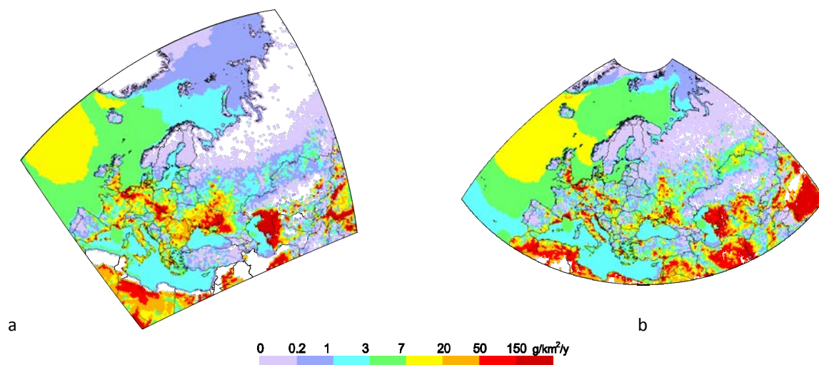
Fig. 2.6. Annual Cd re-suspension flux in 2014 simulated over the old (a) and new (b) EMEP domains
