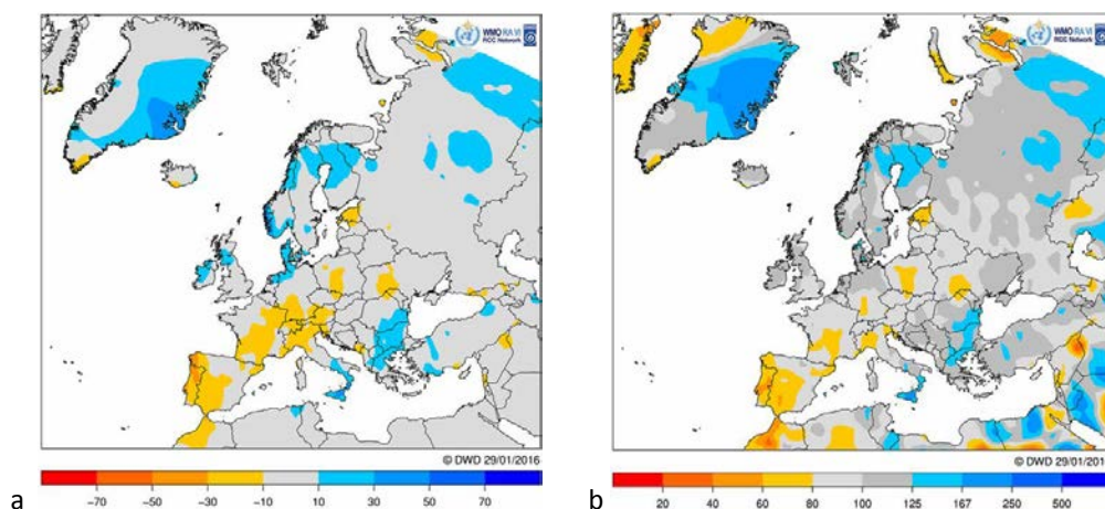
Fig. B.2. Absolute (a, mm/month) and relative (b, %) anomaly of annual precipitation sums in 2015 relative to climatic mean value for the period from 1951 to 2000. Source: http://www.dwd.de/rcc-cm
