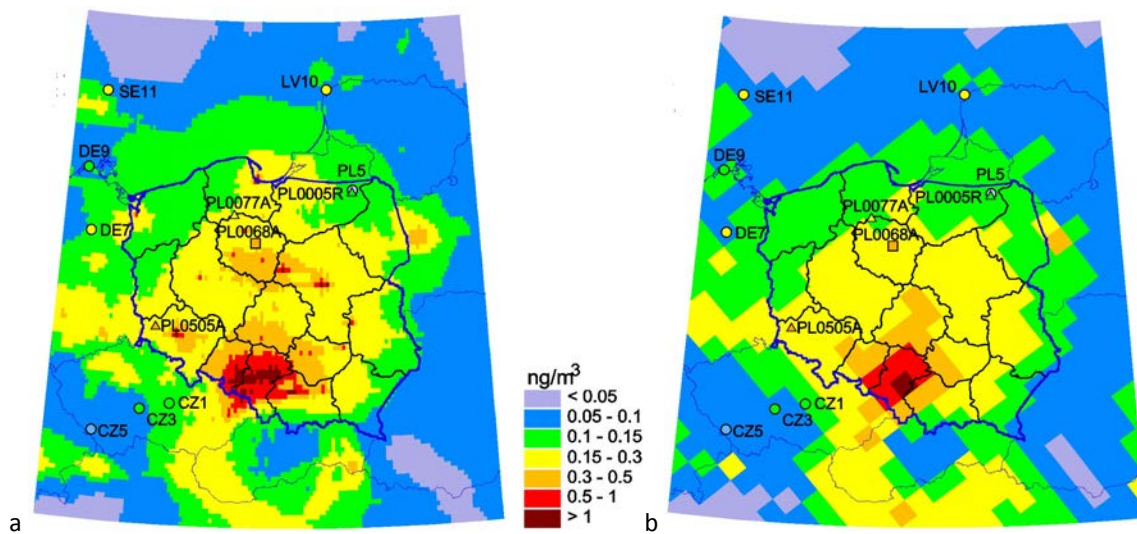
Fig. 3.6. Mean annual modelled concentrations in air on new (a) and old (b) grid and observed concentrations at EMEP (circles), regional background (triangles) and suburban (squares) stations. Measurements are shown in the same colour palette as modelled concentrations
