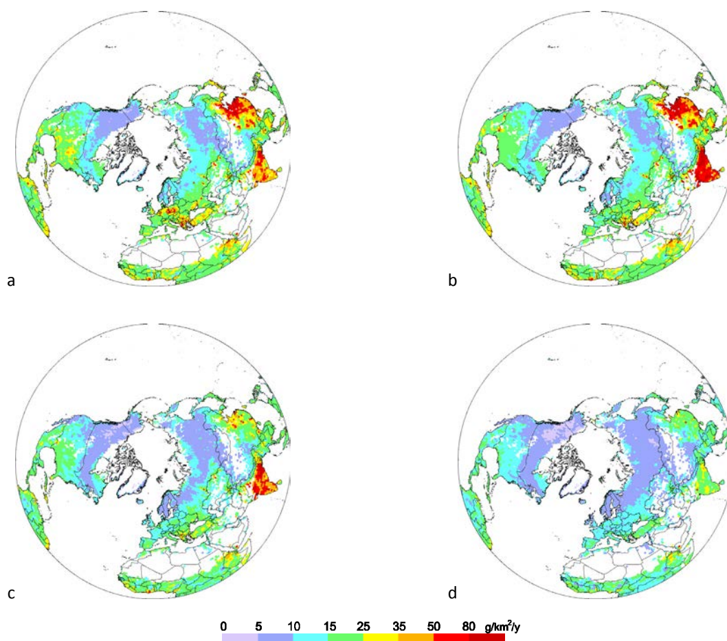
Fig. 4.16. Mercury deposition flux to forests in the Northern Hemisphere in 2010 (a) and in 2035 according to different emission scenarios: (b) – CP 2035; (c) – NP 2035; (d) – MFR 2035
