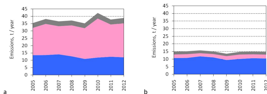
Fig. 3.13. National total emission of cadmium in Poland according to reporting in 2014 (a) and 2017 (b)
