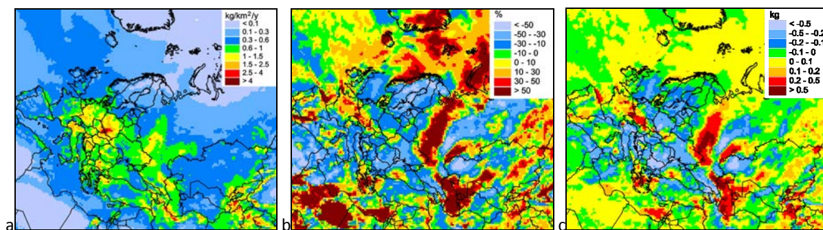
Fig. 1.16. Total deposition of lead in 2015 (a), relative (b) and absolute (c) changes of deposition modelled for 2015 and 2014
