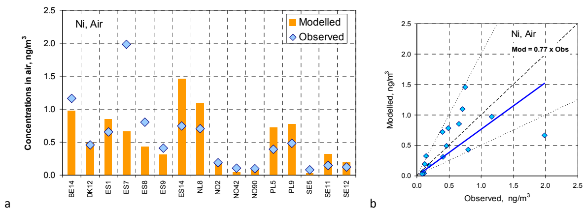
Fig. 4.5. Annual mean modelled and observed concentrations of nickel in air in 2015 at individual stations (a) and their scatter plot (b). Dashed line mean 1:1 ratio, and dotted lines mean 2-fold range
