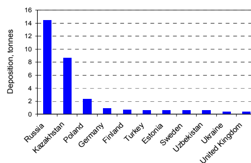
Fig. 1.26. Total deposition of lead caused by emission sources of the EMEP countries to the European and Asian terrestrial areas of the Arctic covered by the EMEP domain. Ten main countries-contributors are shown
