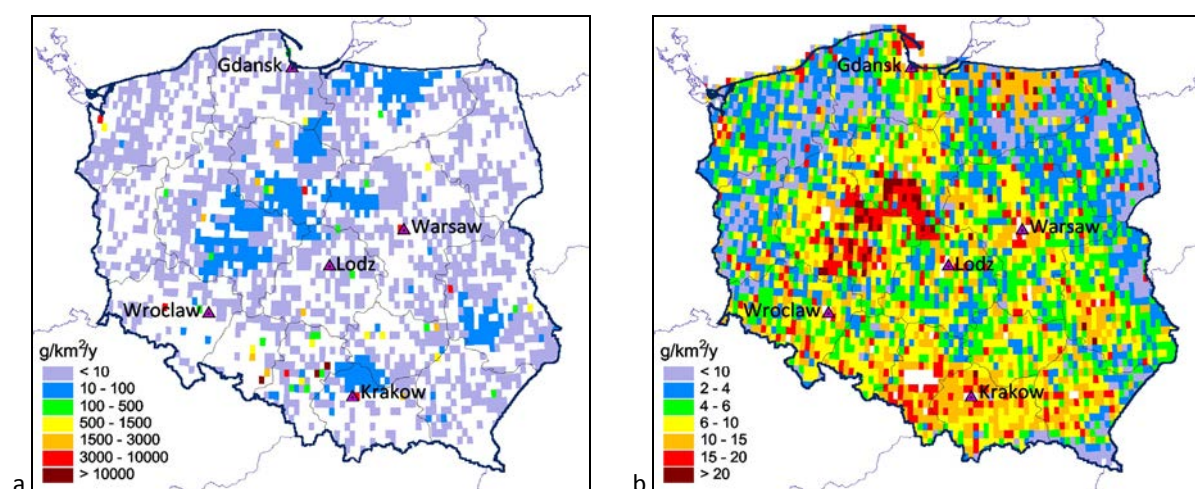
Fig. 3.3. Spatial distribution of cadmium emission in Poland from source categories “Industry” (a) and “Other Stationary Combustion” (b) in 2014. Please note that colour palettes of these two maps are different
