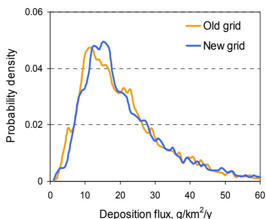
Fig. 2.11. Probability distributions of Cd deposition flux to croplands over the old and new grids
