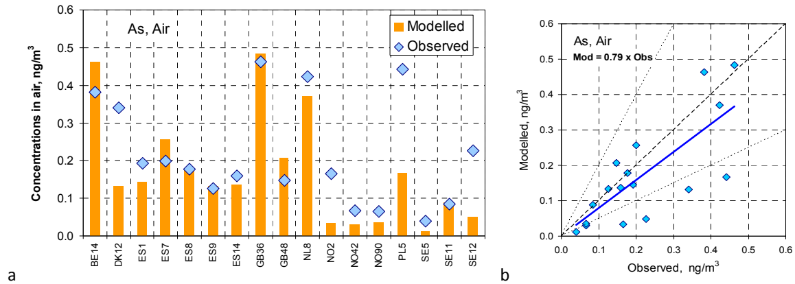
Fig. 4.4. Annual mean modelled and observed concentrations of arsenic in air in 2015 at individual stations (a) and their scatter plot (b). Dashed line mean 1:1 ratio, and dotted lines mean 2-fold range
