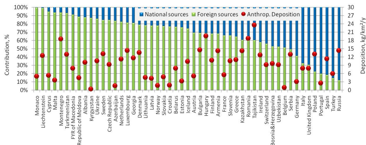
Fig. 1.12. Relative contribution of the transboundary transport and national sources to anthropogenic cadmium deposition in the European and the Central Asian countries and deposition values from anthropogenic emission sources in 2015
