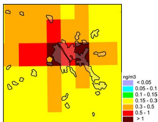
Fig. 3.21. Mean annual concentrations of cadmium in and around Warsaw city. Pentagon indicates location of measurement station PL0214A
