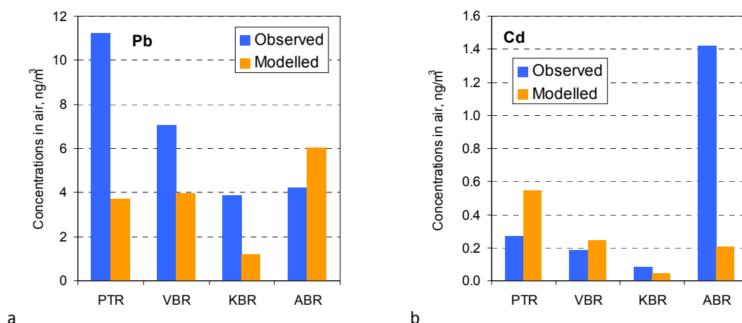
Fig. 4.10. Annual mean modelled and observed concentrations of lead (a) and cadmium (b) at stations of Russian monitoring network in 2014
