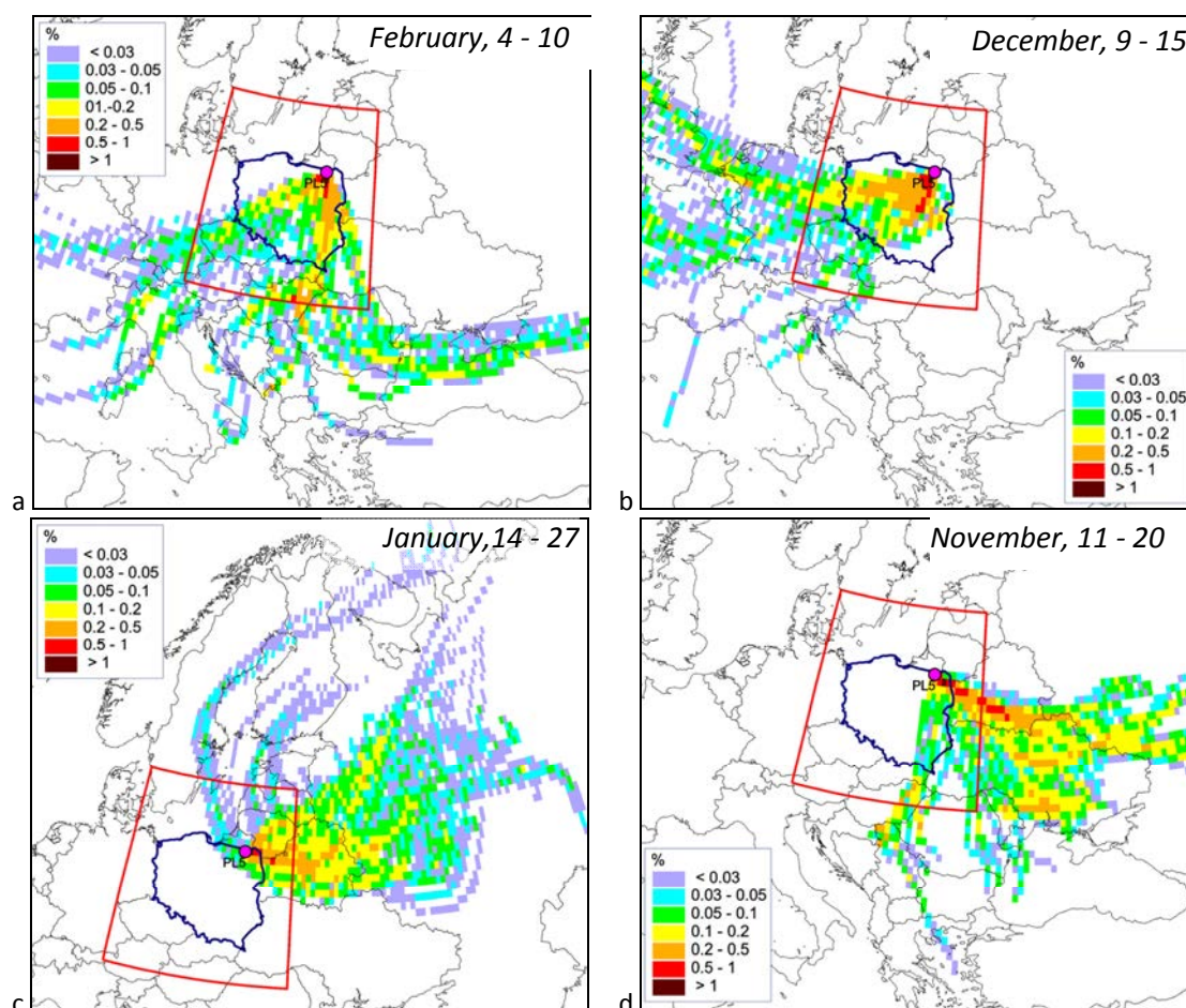
Fig. 3.17. HYSPLIT-based back trajectories (expressed as frequencies of trajectory presence in grid cells) for the EMEP station PL5 (Diabla Gora) for the periods with low (a,b) and significant (c,d) discrepancies between modelled and observed concentrations of cadmium in air
