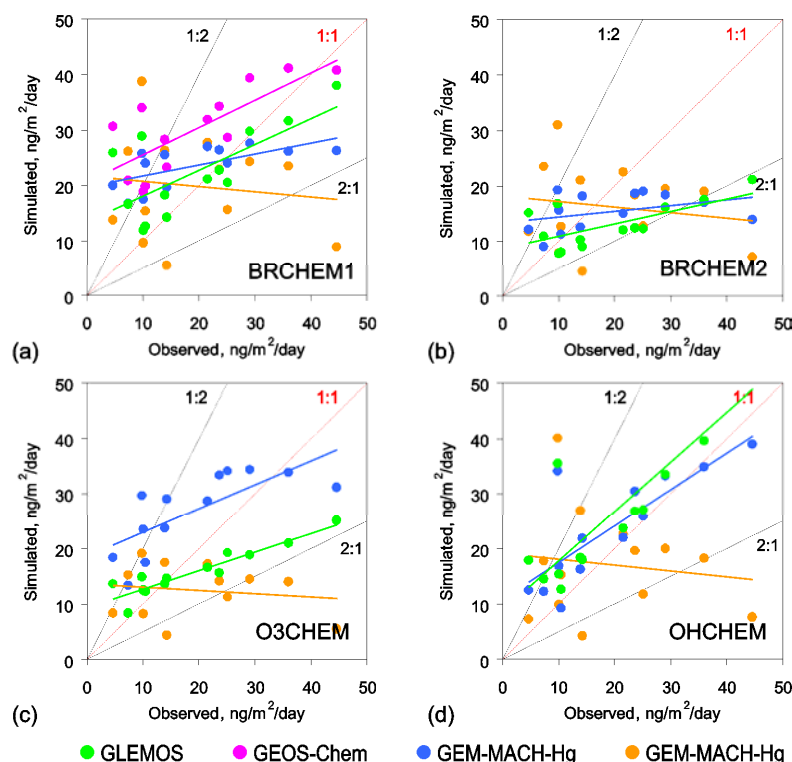
Fig. 2.12. Scatter plots of simulated vs. observed annual mean wet deposition flux in 2013 averaged over different territorial groups of sites for different model experiments: (a) BrCHEM1, (b) BrCHEM2, (c) O3CHEM, and (d) OHCHEM. Solid lines depict linear approximation. Dotted red line depicts the 1:1 ratio; dotted black lines show deviation by a factor of 2
