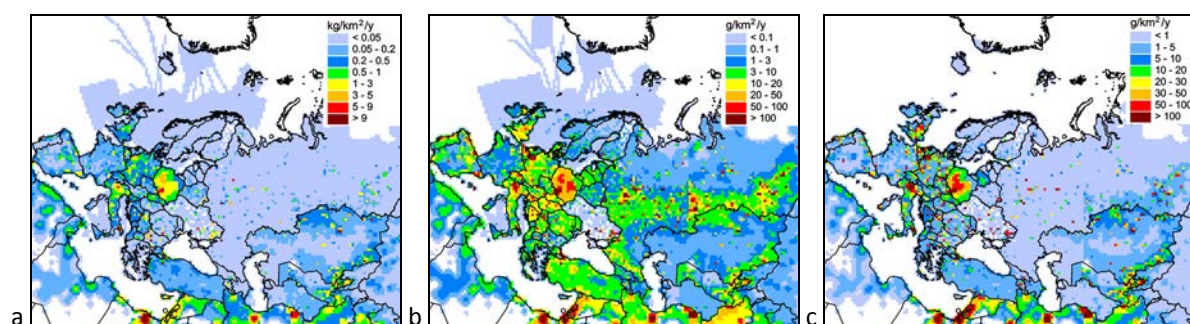
Fig. 1.2. Spatial distribution of lead (a), cadmium (b) and mercury (c) anthropogenic emissions over the EMEP domain in 2015
